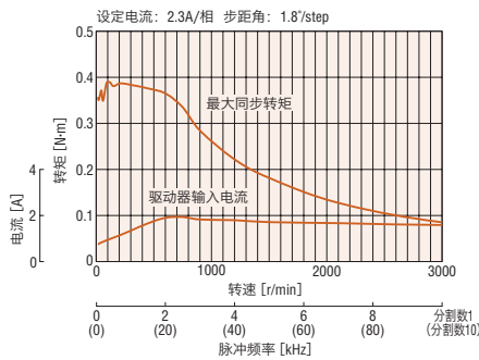
CVK245AK/CVK245BK
